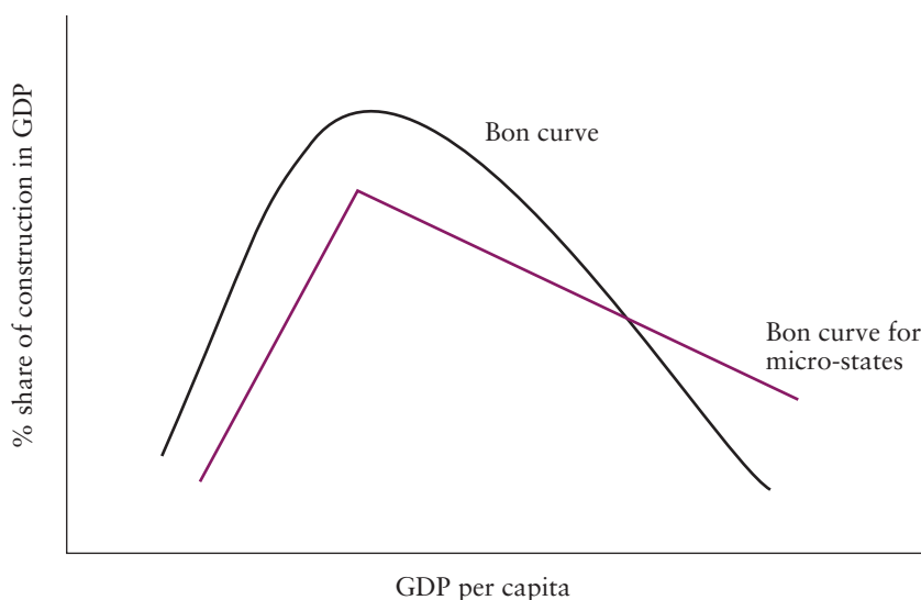
Figure 2 Bon curve for micro-states
