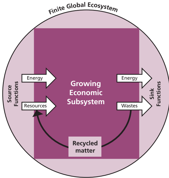
Figure 11.4 Full world
