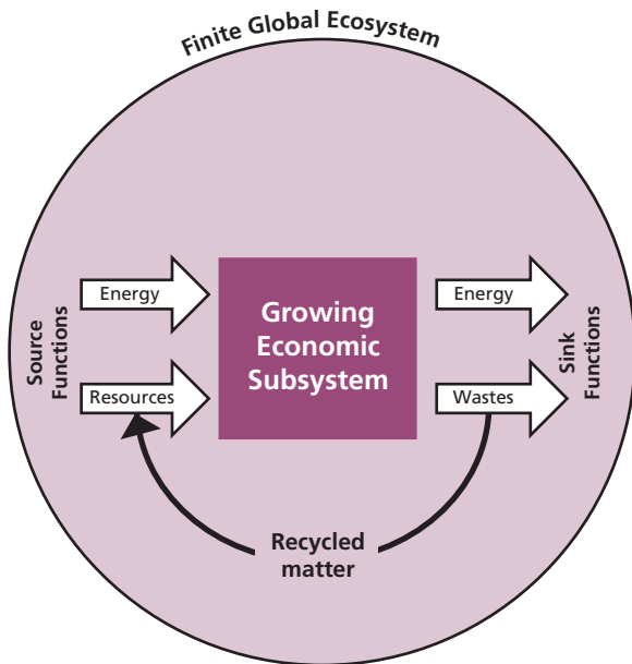
Figure 11.3 Empty world
