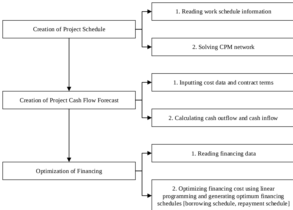
Figure 1. Model Algorithm
