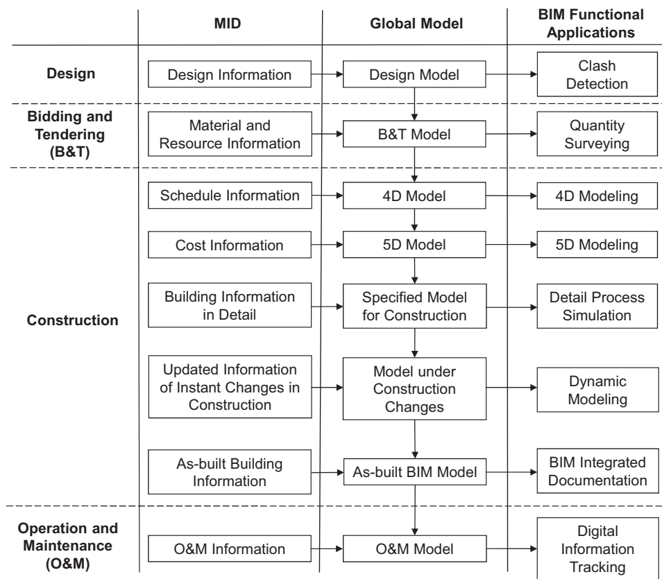
Fig. 4. BIM roadmap of the project lifecycle. (Adapted from Ma et al. 2015.)
