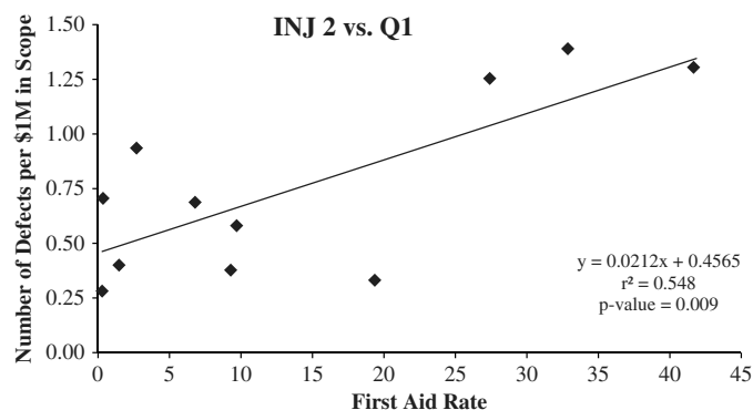
Fig. 3. First aid rate per 200,000 worker-hours (INJ2) versus the number of defects per $1 million project scope completed (Q1)
